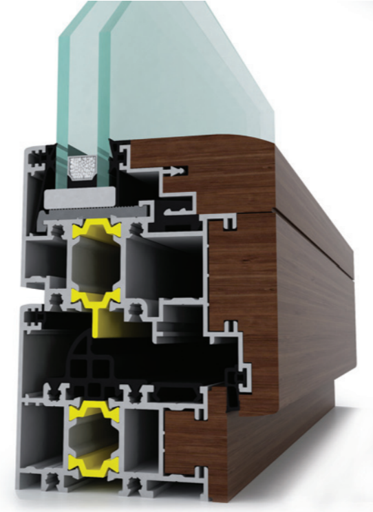
altimba 81 U_{min} : 1,43 \text{ W/m}^2\text{K}
